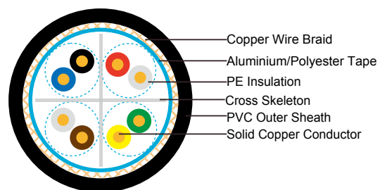
SF/UTP CAT6
