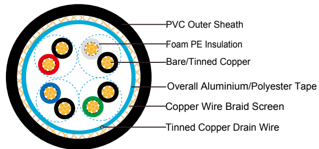
RS 485
